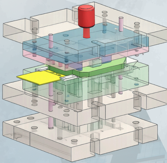
DIES PROGRESIF
